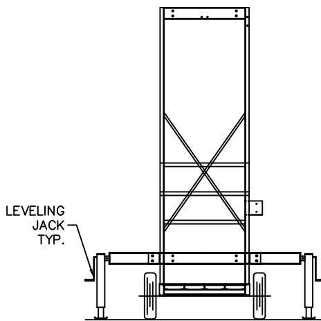
FRONT VIEW LADDERS NOT SHOWN
